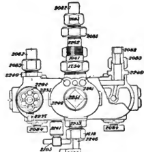
Fig. 3197. Plan View.
